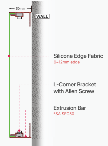
Side View : Wall Mounted
